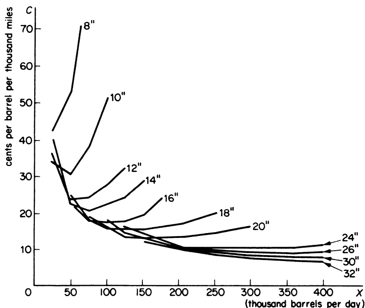
Figure 4.44 Costs per barrel of operating crude-oil trunk pipelines.
